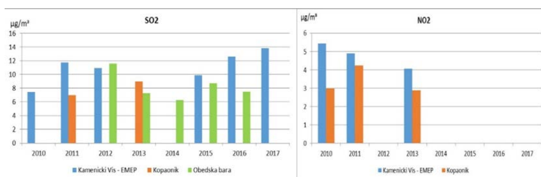
Fig. 1.1.3.1. Trend of \text{SO}_2 and \text{NO}_2 in the selected protected areas
